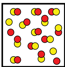
Mostly diatomic molecules:
