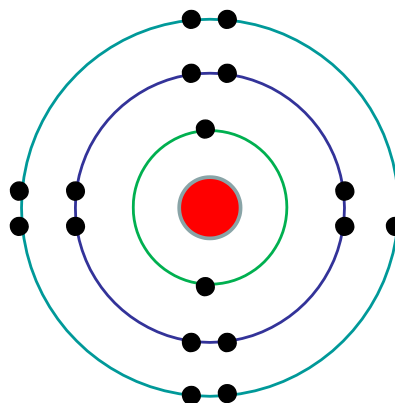
The outer electrons of a Chlorine atom feel an effective nuclear charge of 17 - 10 = 7
