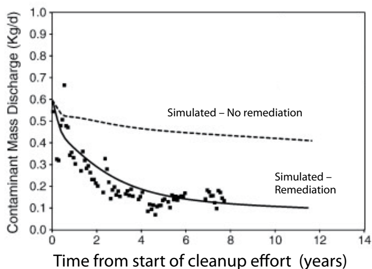
Figure 9.7 Model predictions for TCE at the Tucson airport site with remediation (solid line) and without remediation (dotted line). The mass of TCE removed over the first eight years are shown with dots. Time = 0 is the start of the cleanup effort.
