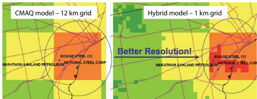
Figure 7.7 The AERMOD model uses a 1 \text{ km} \times 1 \text{ km} grid size, compared with 12 \text{ km} \times 12 \text{ km} for the CMAQ model. This provides 144 AERMOD receptor estimates for each CMAQ estimate, and these are for different pollutants. The hybrid approach merges the two outputs and gives better resolution and better management decisions. (Wesson et al 2009, 2010; USEPA 2008)
