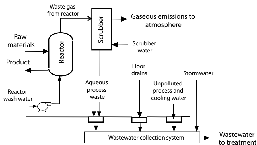
Figure 3.3 Water use in the manufacturing process. Wastewater consists of process waste, water used for cleanup and for air pollution control, drainage from floors, as well as unpolluted process and cooling water and stormwater. This diagram, for simplicity, shows all wastewater going into a common drain. Better practice is to segregate (i.e. collect separately) different kinds of wastewater. For example, do not mix unpolluted water with polluted water.
