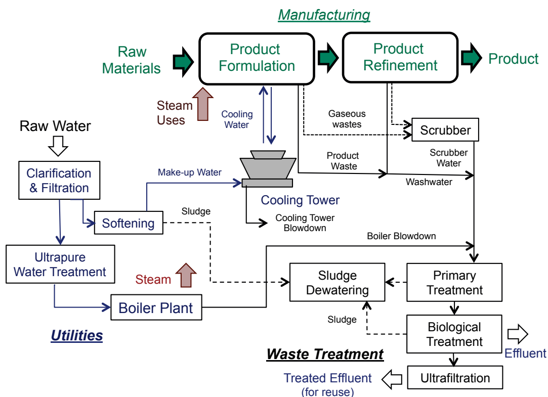
Figure 3.4 The Industrial Water Cycle. Industries run on water and energy as much as on raw materials used in the actual manufacturing. Water for the formulation and refinement of the product is supplied from plant utilities, which also supplies boilers and cooling towers. Wastewater streams include blowdown from boilers and cooling towers, scrubbers, and waste from manufacturing, including washwater. Water treatment and wastewater treatment produce sludge. There may also be solid wastes (not shown) from manufacturing. Waste treatment may be done off-site at a municipal treatment plant, but on-site treatment will offer more opportunities to recycle water.
