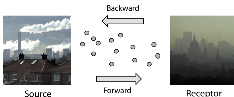
Figure 7.6 A receptor model can be run forward or backward in time to predict source emission or conditions at the receptor.
