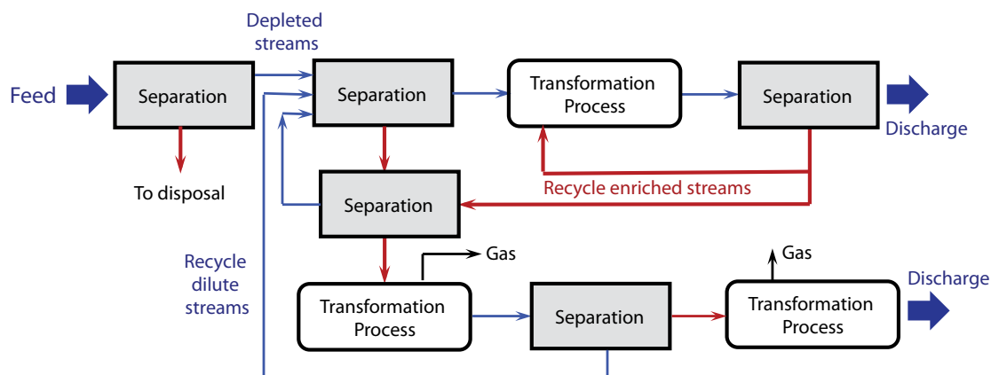
Figure 1.7 A generic integrated system that includes transformations and separations.
