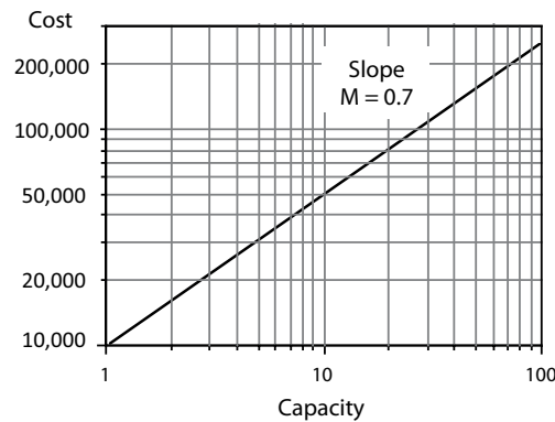
Figure 2.7 Economy-of-scale cost function used for making preliminary cost estimates. This curve is for a hypothetical machine that is used for pollution control. C = \$10,000Q^{0.7} where Q = design capacity (volume, area, flow rate, etc.)
