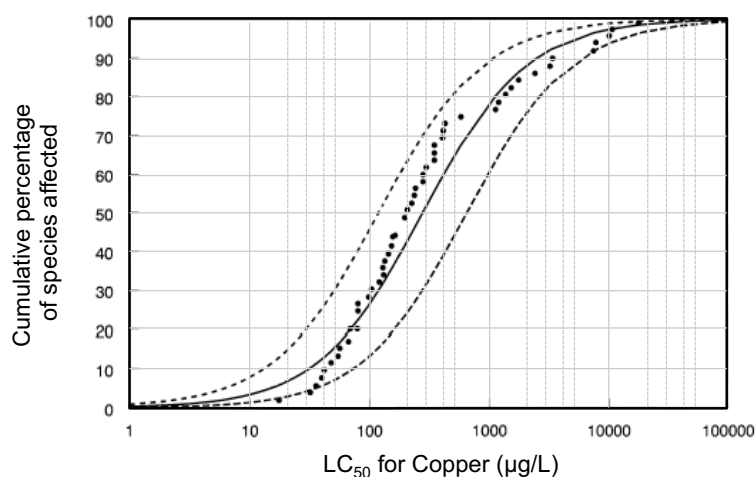
Figure 4.3 Species sensitivity to copper.
