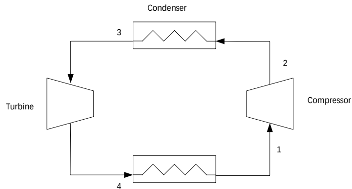
Figure 5.18: Air-standard refrigeration cycle.
