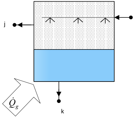
Figure 6.6: Generator element.
