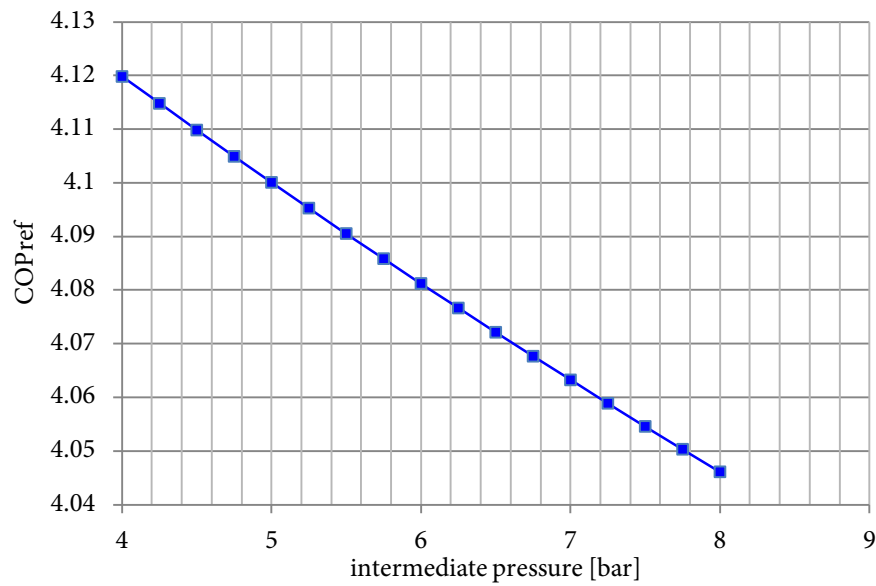
Figure 7.16: Refrigeration COP against intermediate pressure. The evaporator pressure is set to 1.33 bar and the high pressure condenser at 10 bar. The lower stage mass flow rate is set to 1 kg/s while the higher stage compressor is set to 0.8 kg/s.
