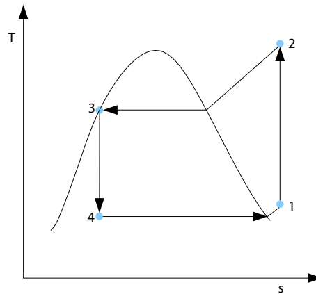
Figure 4.2: Modified Carnot cycle with superheated vapour at compressor inlet.
