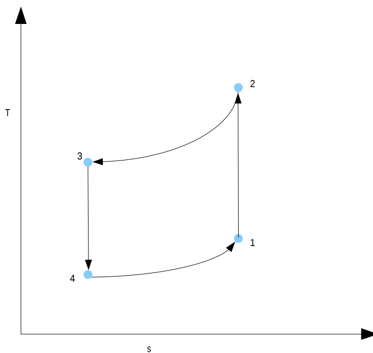
Figure 5.19: Air-standard refrigeration cycle T-s diagram.
