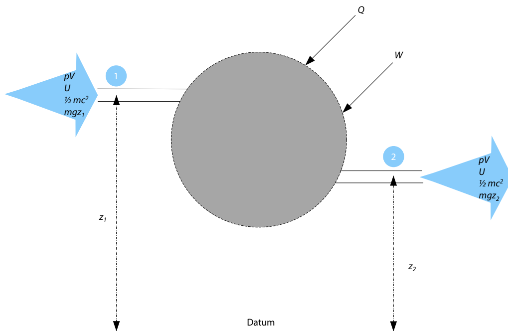
Figure 1.7: Steady flow thermodynamic system showing energy inputs and energy outputs at the inlet (1) and outlet (2).
