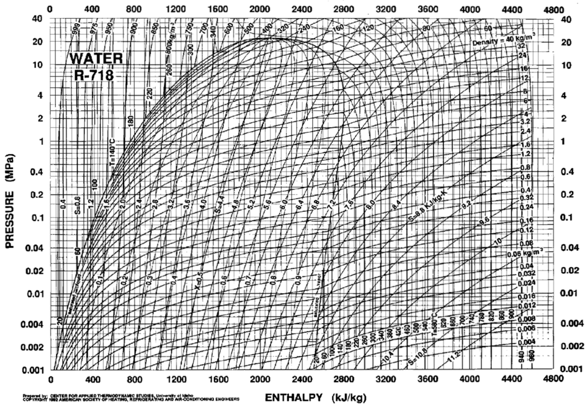
Figure A.5: p-h diagram for refrigerant R718 water/steam ASHRAE (2009) . ©ASHRAE, www.ashrae.org . 2009 ASHRAE Handbook – Fundamentals.
