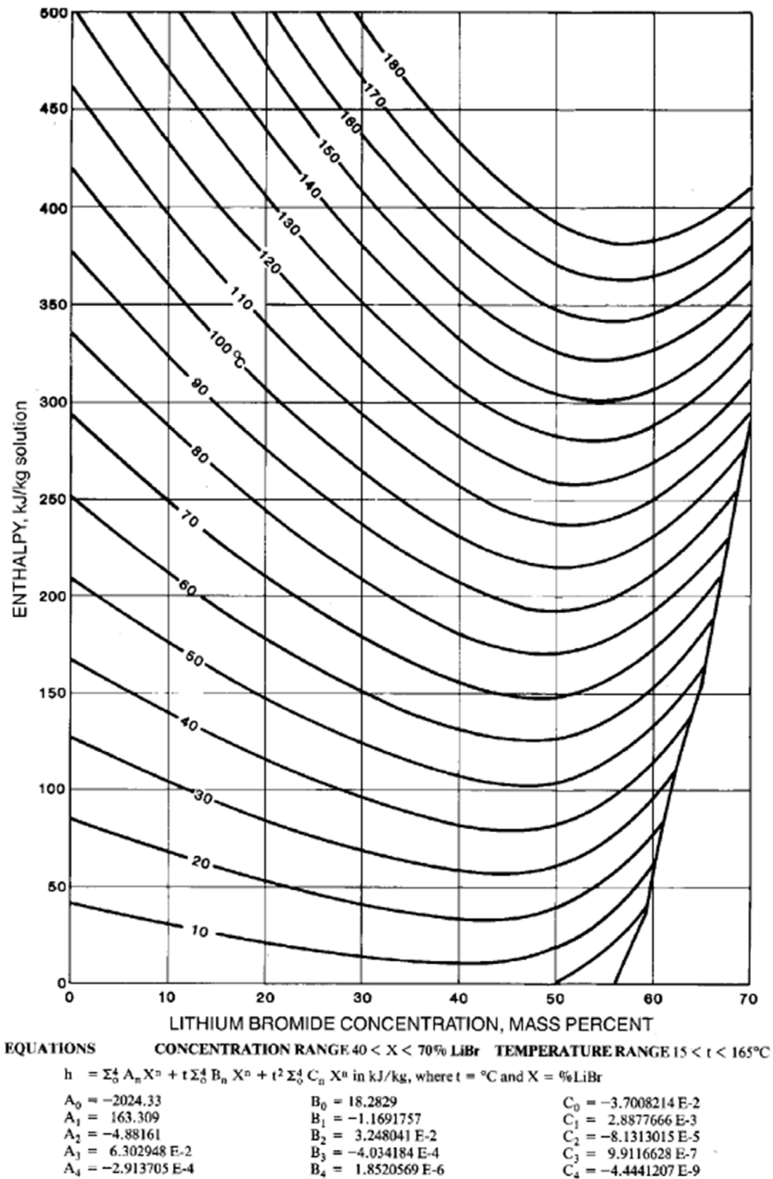
Figure A.10: Enthalpy concentration chart for water-LiBr solutions ASHRAE (2009). ©ASHRAE, www.ashrae.org . 2009 ASHRAE Handbook – Fundamentals.
